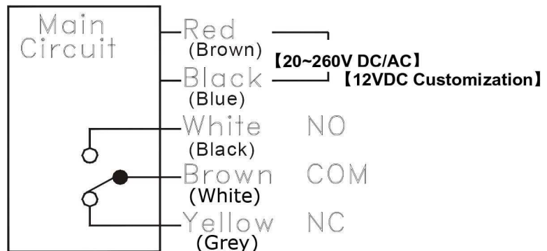
Connection diagram
